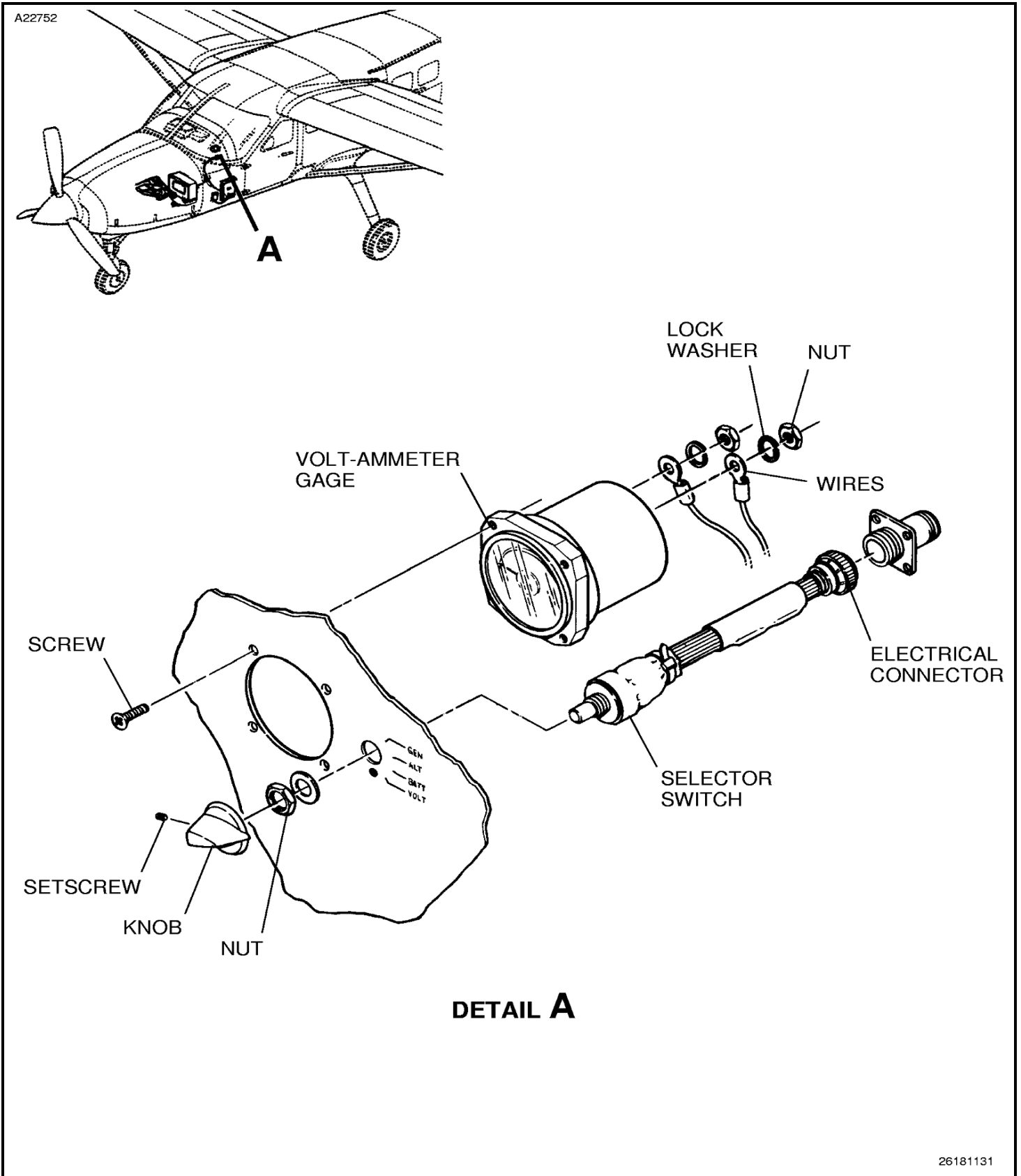
Figure 201 : Sheet 1 : Electrical Monitoring Installation
